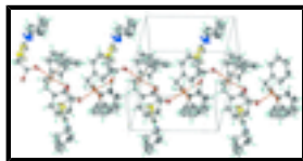
Fig. 3. Anisotropic displacement ellipsoid plot (Barbour, 2001) of the chain structure of polymeric \text{Sn}(\text{C}_7\text{H}_7)_3(\text{C}_8\text{H}_{12}\text{NO}_2\text{S}_2) at the 50% probability level. Hydrogen atoms are drawn as spheres of arbitrary radius.
